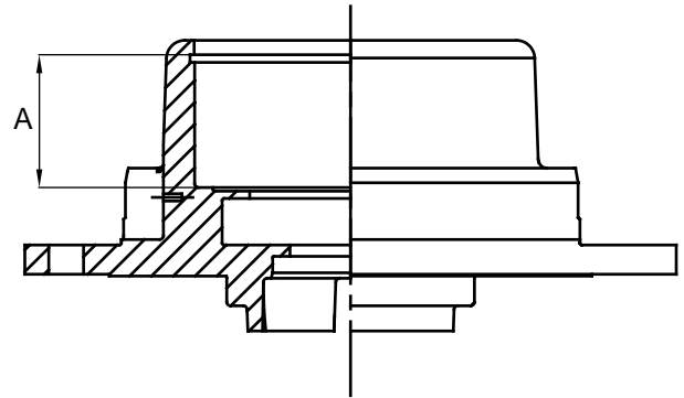
A = 72,5 mm Bearing holder, part No 50 418 02
